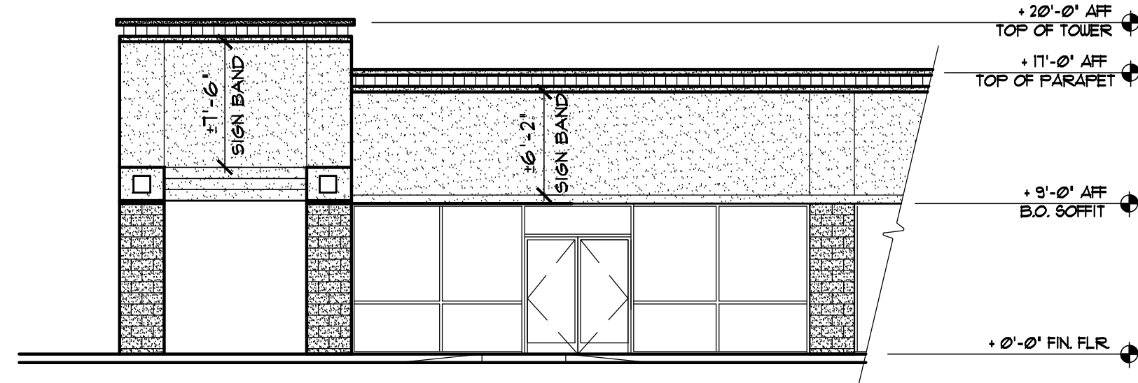
3 ext. elev. (east) - ste. 7895
