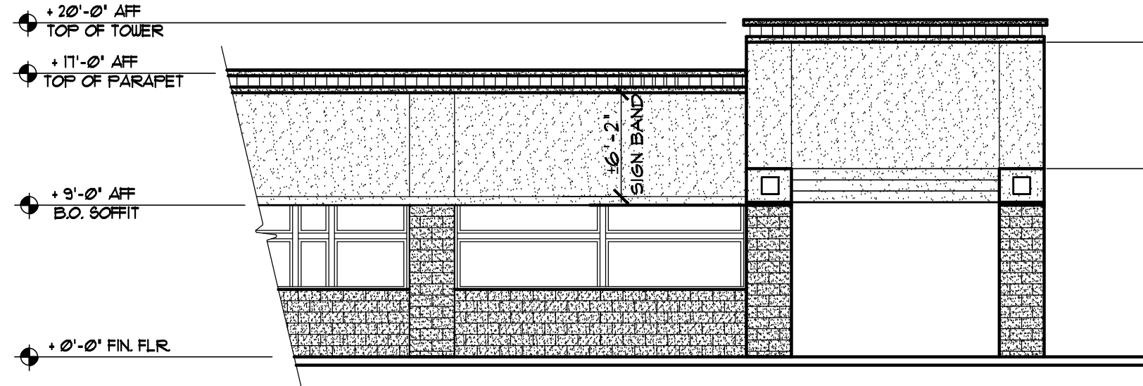
2 ext. elev. (south) - ste. 7895
