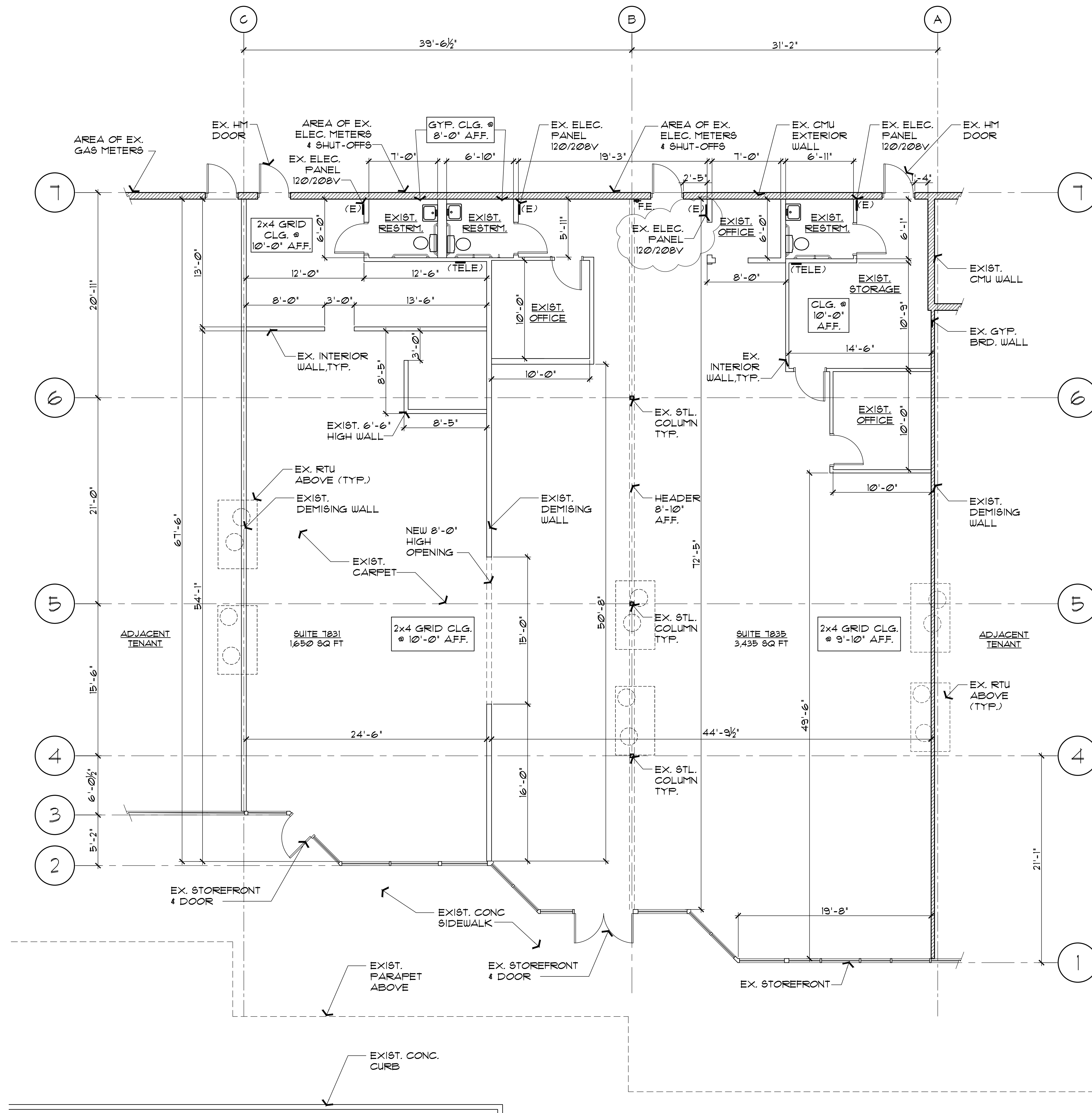
1 floor plan - suites 7831 & 7835
