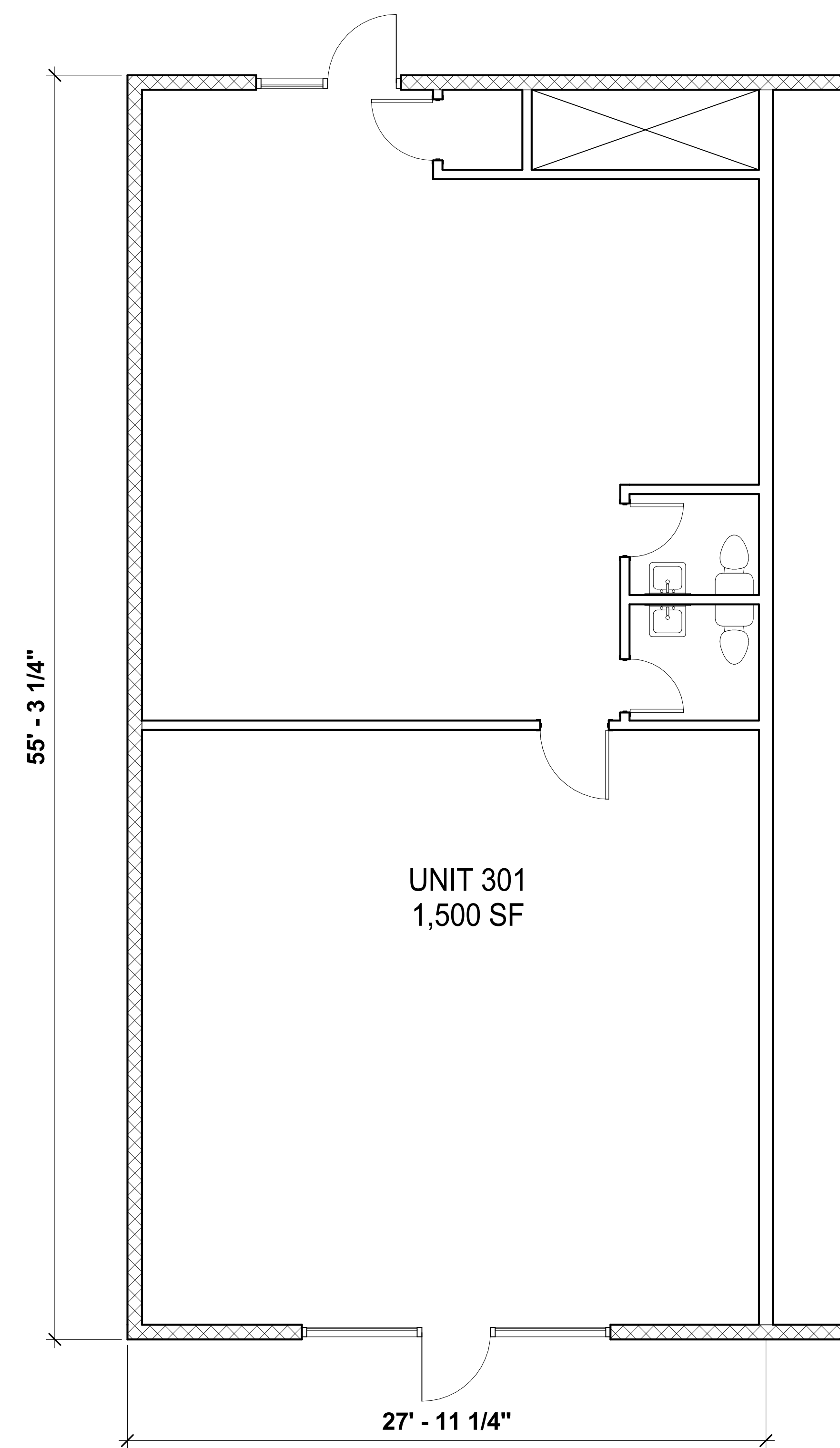
③ 301 LEASE OUTLINE DRAWING 1/4" = 1'-0"
